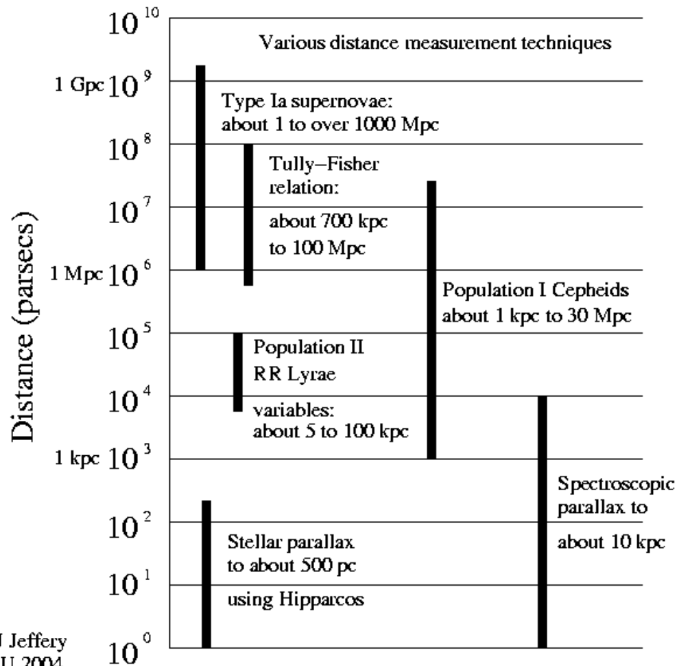
A Cartoon of the Distance Ladder
